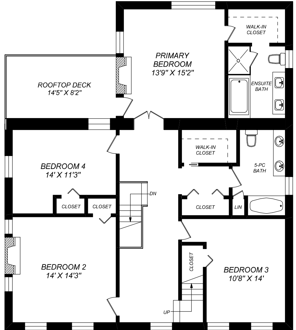
SECOND FLOOR 1484 SQUARE FEET CEILING HEIGHT : 8'-6"
