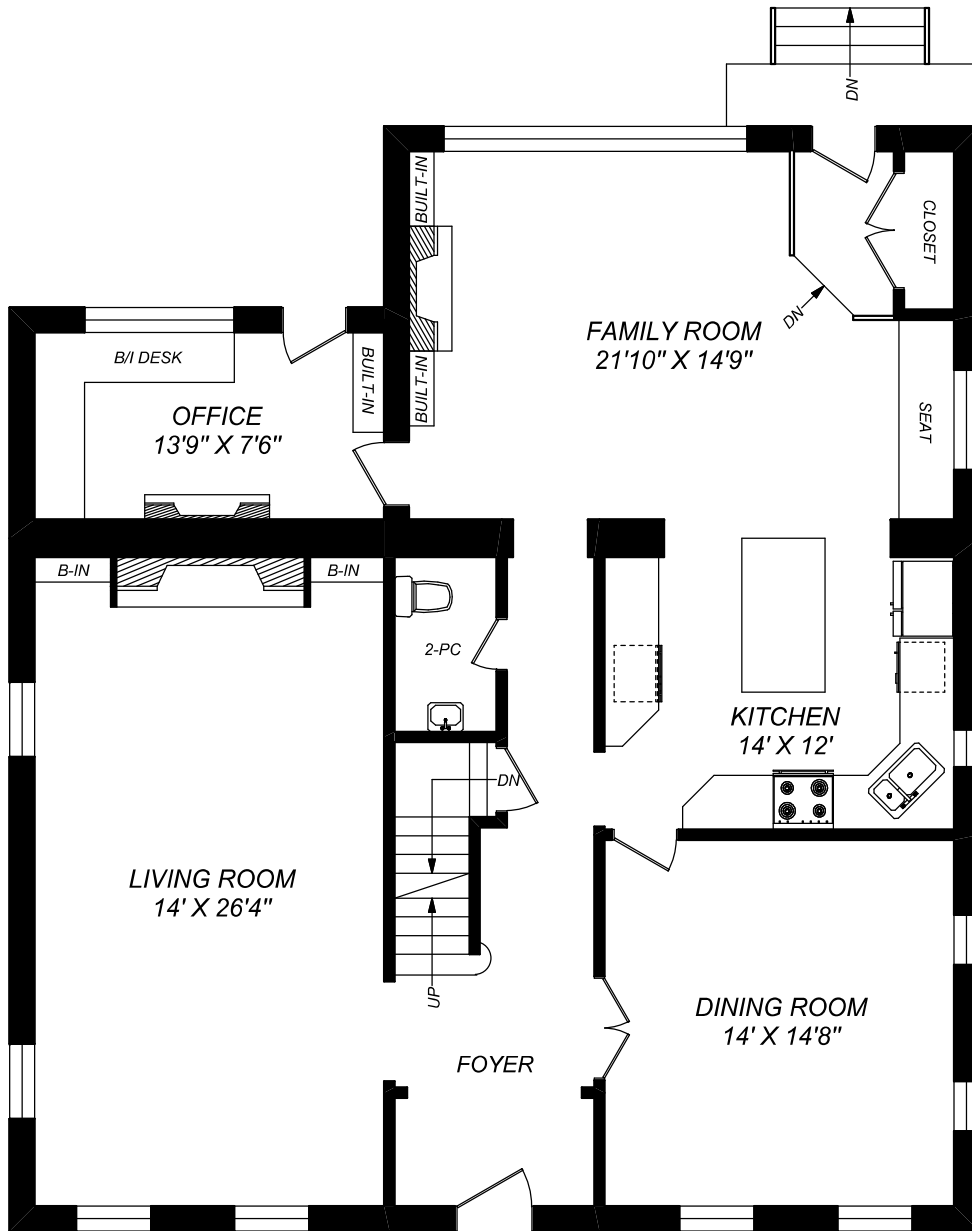
MAIN FLOOR 1610 SQUARE FEET CEILING HEIGHT : 8'-6"
